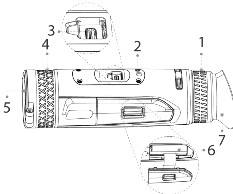
Figure 2-4 Port description
